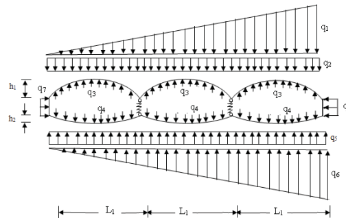
Fig.5 Multi-arch and loading distribution map
