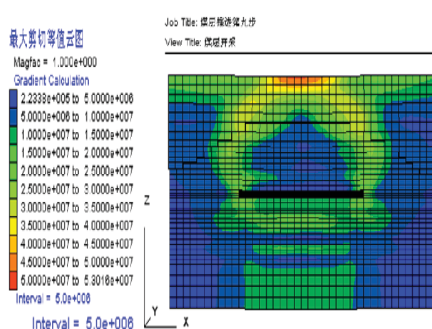
Fig.17 the maximum shear stress cloud when mined to 90m
